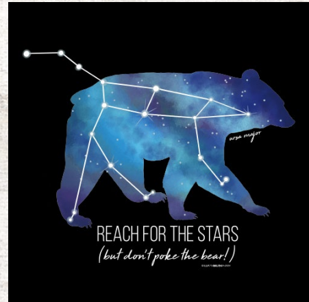
703 - URSA MAJOR
